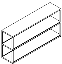
COMBINATION 202 Width 150 cm Depth 34 cm Height 74 cm
