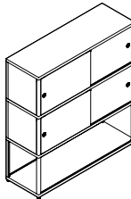
COMBINATION 305 Width 100 cm Depth 34 cm Height 109,3 cm
