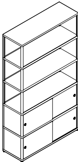
COMBINATION 503 Width 150 cm Depth 34 cm Height 179,9 cm
