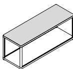
COMBINATION 100 | BENCH Width 100 cm Depth 34 cm Height 38,7 cm
