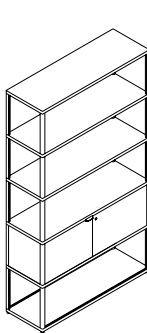
COMBINATION 502 Width 100 cm Depth 34 cm Height 179,9 cm
